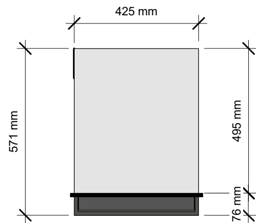
① TOP VIEW 1 : 12
