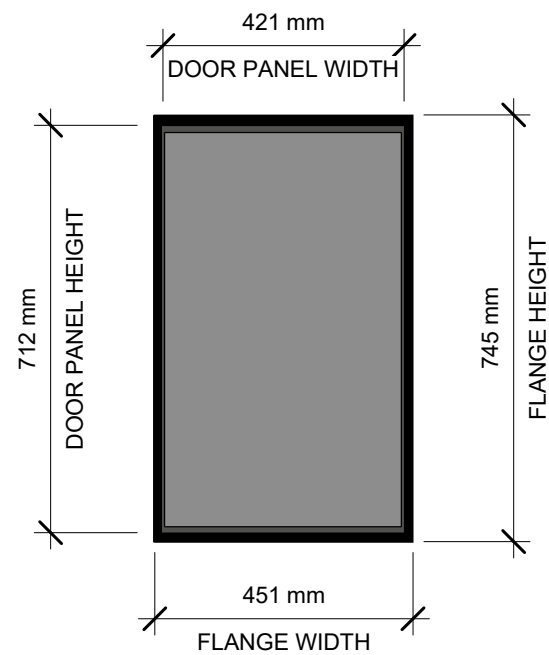
③ FRONT VIEW 1 : 12
