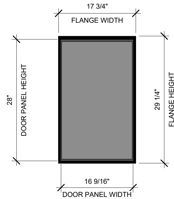
③ FRONT VIEW 1" = 1'-0"
